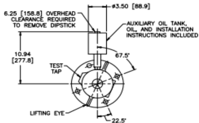
FLANGE ALIGNMENT DIAGRAM - TOP VIEW SHOWN HORIZONTALLY MOUNTED
